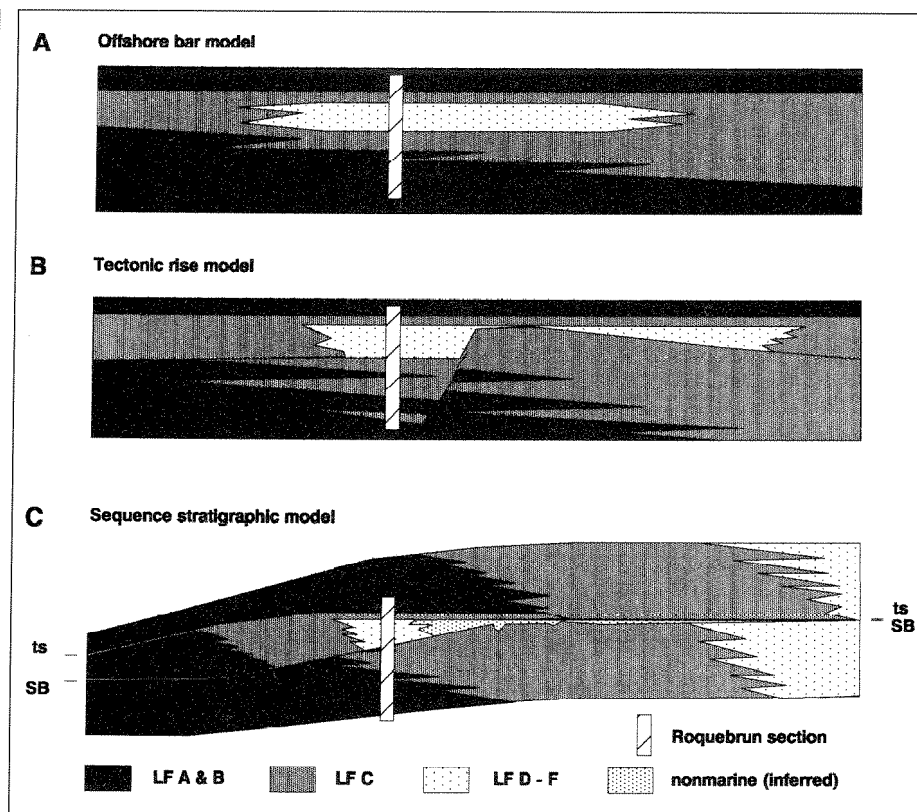
Fig. 13. – Diagrammatic comparison of the lithostratigraphic models for the Roquebrun series as discussed in the text. Note that the original geometry of the Cluse de l'Orb Fm. (LF D-F) is reconstructed different in either model. SB: sequence boundary, ts: transgressive surface. In the sequence stratigraphic model (C), nonmarine deposits or paleosols are inferred, as a working hypothesis, to the south of the Montagne Noire, e.g. on the Saharan platform.
