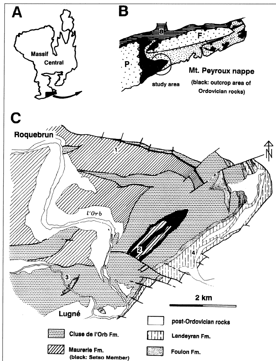
Fig 1. A,B. – Tectonic sketch map of eastern Montagne Noire and location of the study area; a: autochthon/parautochthon, F: Mts. de Faugères Nappe, P: Pardailhan Nappe (Arthaud, 1970; Engel et al. , 1981). C: Simplified geological map of the Ordovician rocks of the Roquebrun Synform (after Noffke 1992). The whole sequence is tectonically inverted. Numbers 1-4 refer to outcrops cited in Fig. 11.
