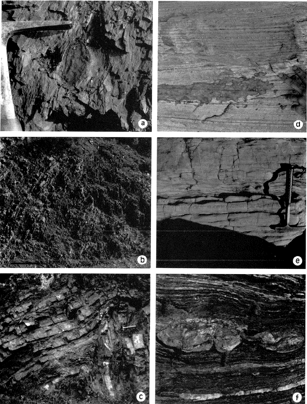
Plate 1. – Lithofacies types of the Ordovician rocks near Roquebrun.
