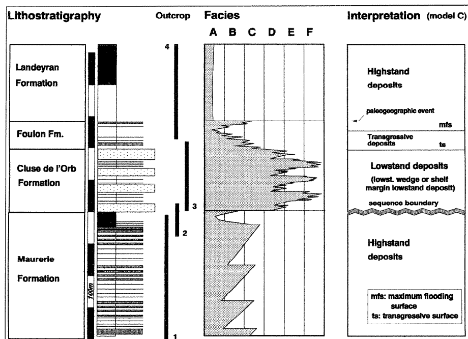
Fig. 11. – Composite log and facies distribution for the upper 900 m of the studied section. Lithofacies types range from A (open shelf, most distal) to F (lagoonal, most proximal). Quartzitic "Lingula-Sandstones" (wide stipple) display complex facies architecture predominantly of LF D and E (see Fig. 9). Note that the shale-sandstone alternations of the Cluse de l'Orb Fm. are composed of LF F (with minor portions of LF E), but those of Maurerie and Foulon formations belong to LF A to C, respectively. Outcrop bars designate: 1. Route de Laurenque, 2. Setso Valley, 3. Rieuberliou Valley, 4. Landeyran Valley; (cf. Fig. 1). In a sequence stratigraphic interpretation (model C), the Cluse de l'Orb Fm. is proposed to represent a lowstand shelf margin deposit, superseded by transgressive (thinning upward) Foulon shelf deposits. The maximum flooding deposit is probably positioned within the Foulon Fm. (at the turning point from thinning upward to thickening upward architecture) but may alternatively be hidden within the monotonous, sand-free shales of the Landeyran Fm.
